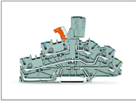
Multilevel installation terminal block (2003-6641) fitted with an N/L-test plug adapter (2003-499) for insulation resistance measurement of the connected N- and L-potentials
