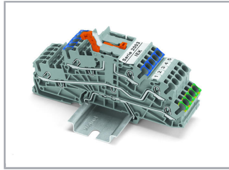
N-potential disconnection via N-knife disconnect within a terminal block assembly without a busbar.
